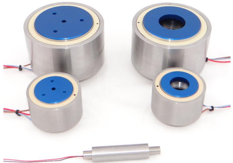
Left: Actuators with threaded holes Right: Actuators with through-hole.
